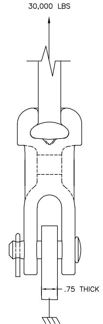
ULT. LOAD DIAGRAM
